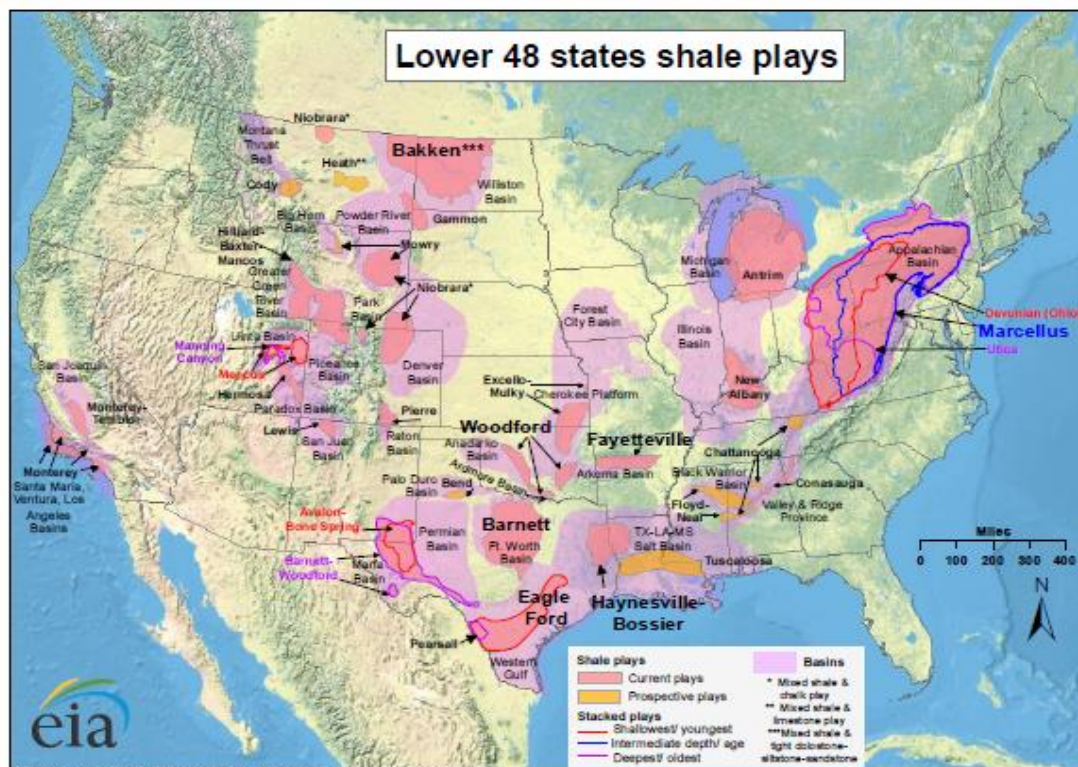
Figure 3.3 – Lower 48 States Shale Plays
