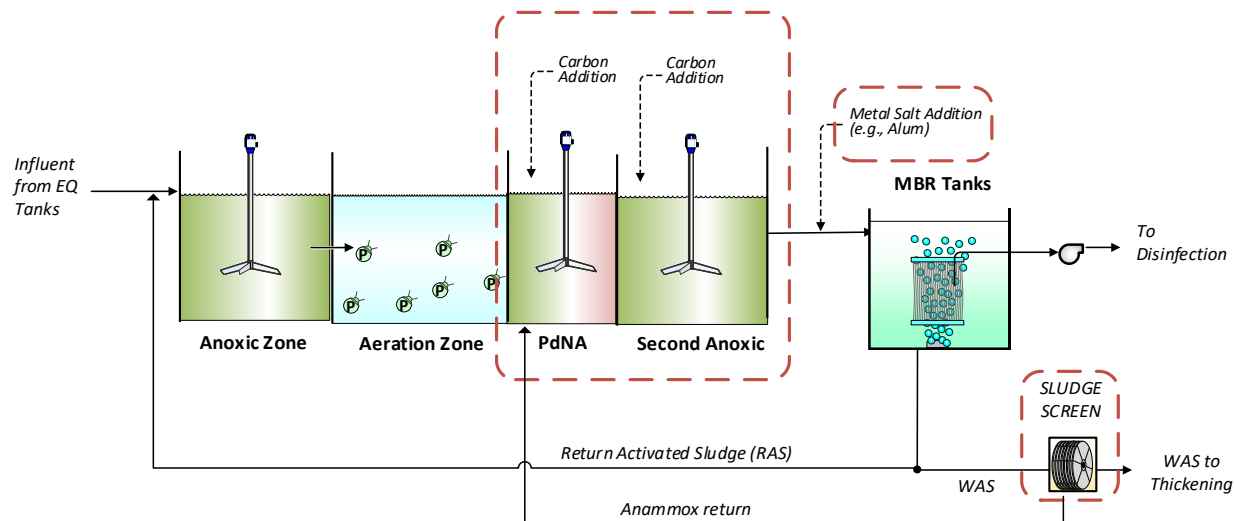
Figure 5-13 AWT Alternative 3 – PdNA + Chem-P PFD
