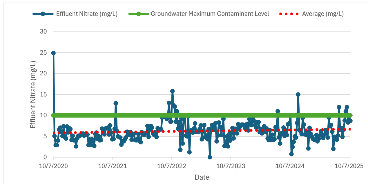
Figure 2-12 Effluent Nitrate (2020 – 2025)
