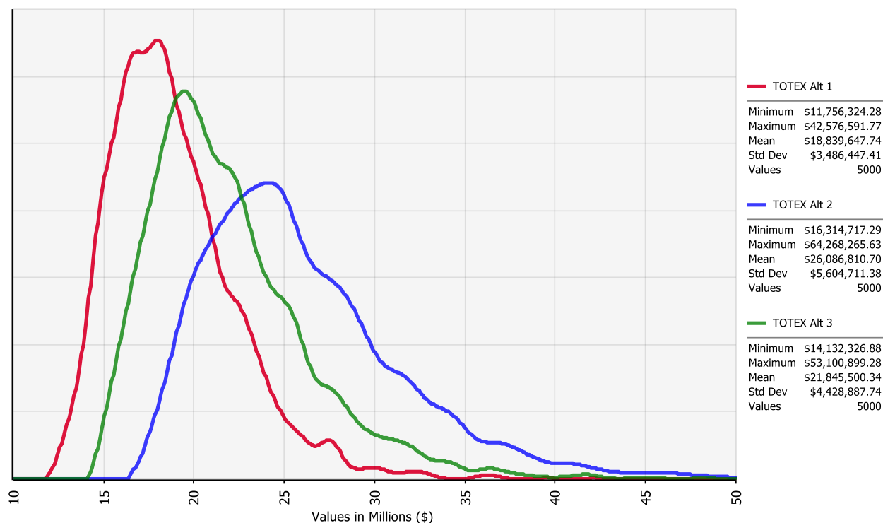
Figure 5-20 AWT Alternatives Combined TOTEX Envelopes – Over a 20 Year Period
