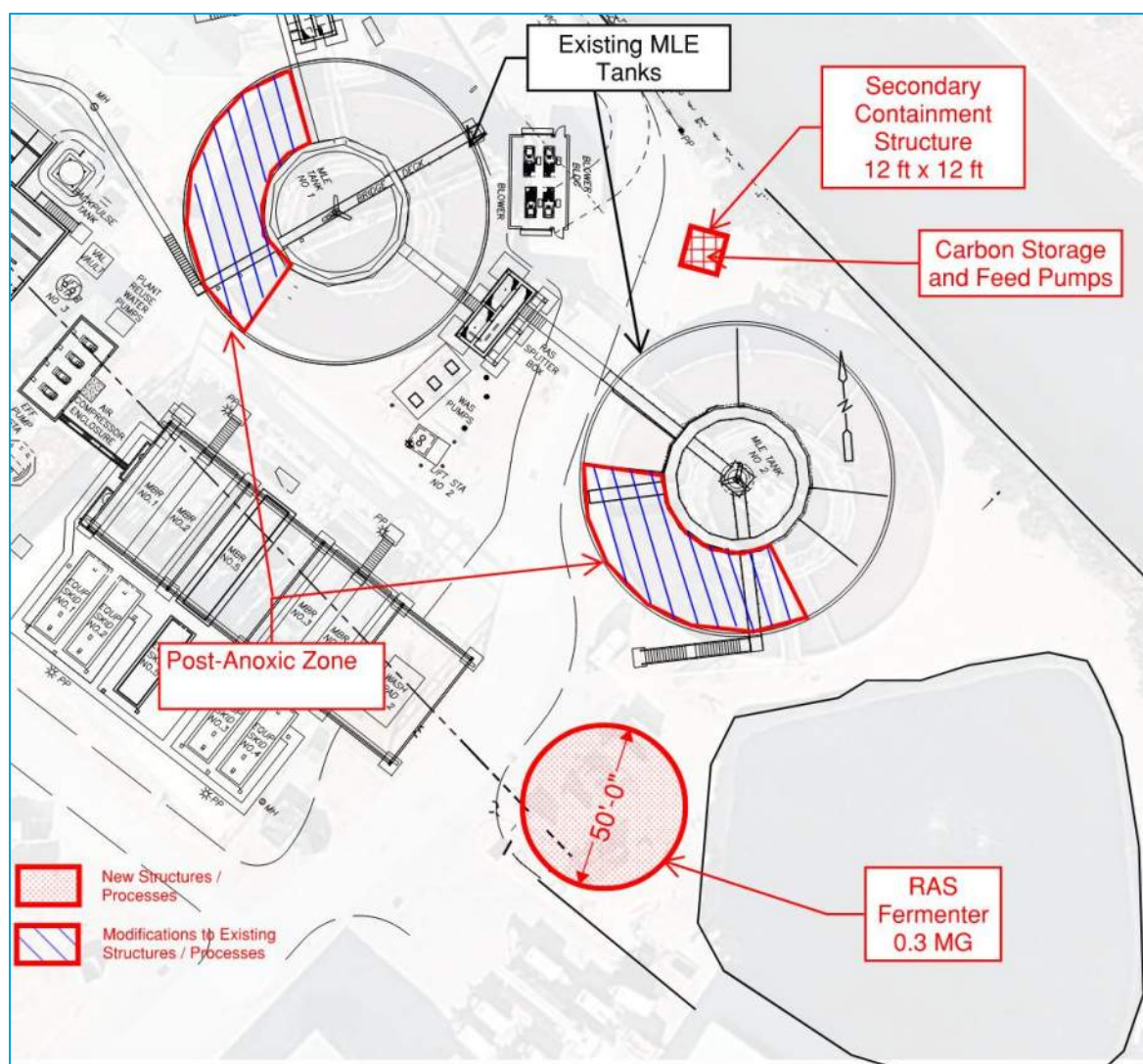
Figure 5-4 Alternative 1 – Four-Stage Bardenpho + S2EBPR – Proposed Site Layout (proposed shown in red)
