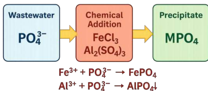
Figure 4-7 Chem-P Removal
