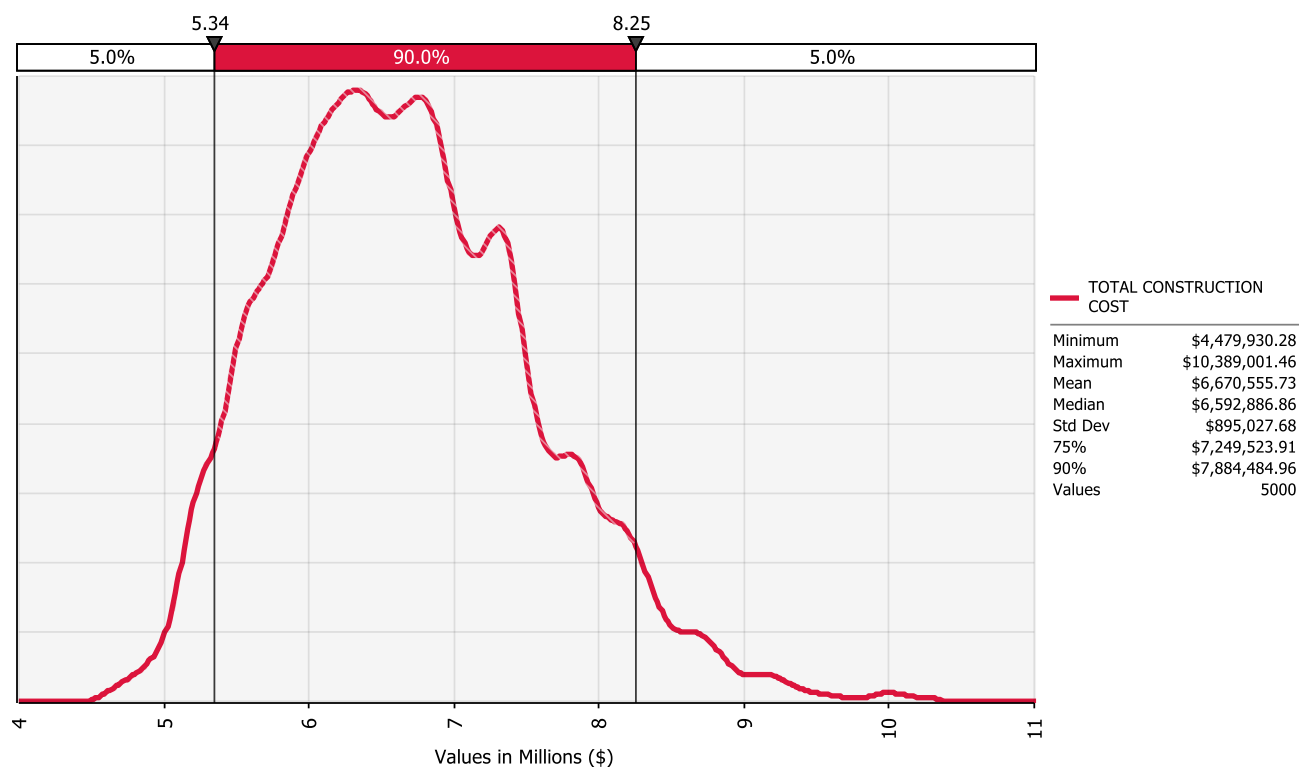
Figure 5-16 AWT Alternative 3 – CAPEX Envelope
