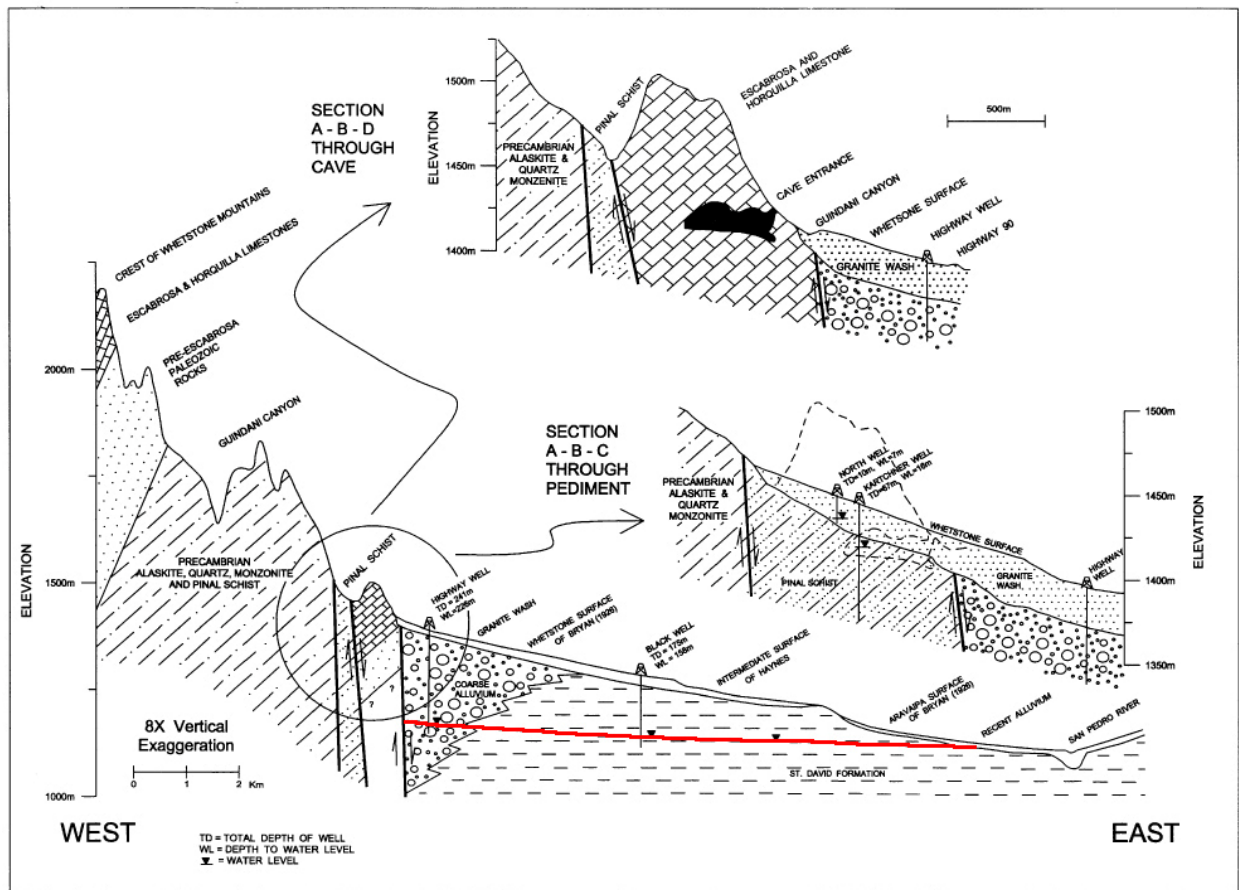
Figure 13. Cross section from the San Pedro River through Kartchner Caverns State Park (Figure 2 from Graf, 1999 ) showing the basin-bounding fault between the Highway Well and the Kartchner block. The downthrown side of the fault contains a thick section of coarse alluvium that led the Kartchner family to think the section might serve as an aquifer for development. The depth to water on the downthrown side of the fault is greater than 700 ft, and pumping capacity appears to be low. The red line is the static water level derived from three wells (denoted by partly covered black triangles).
