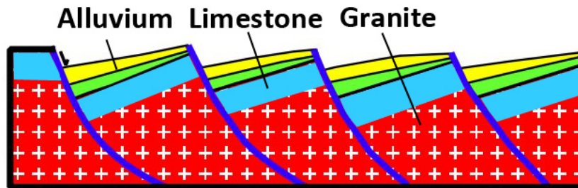
Figure 16. Schematic cross section showing the multiple fault blocks that bound and potentially underlie the west side of the Benson subbasin.
