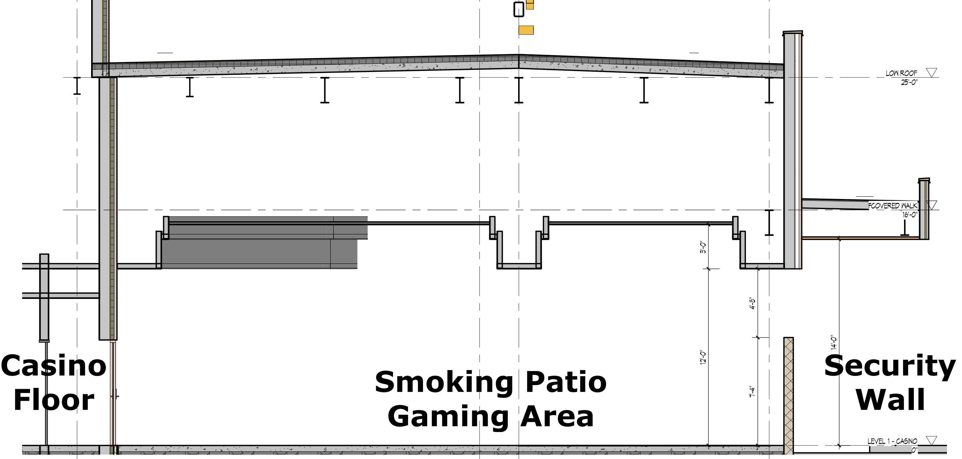
1 SECTION THROUGH OUTDOOR PATIO 5K-002 1/4" = 1'-0"
