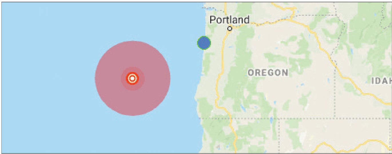
The area of the Saturday morning undersea earthquake west of Coos Bay.
