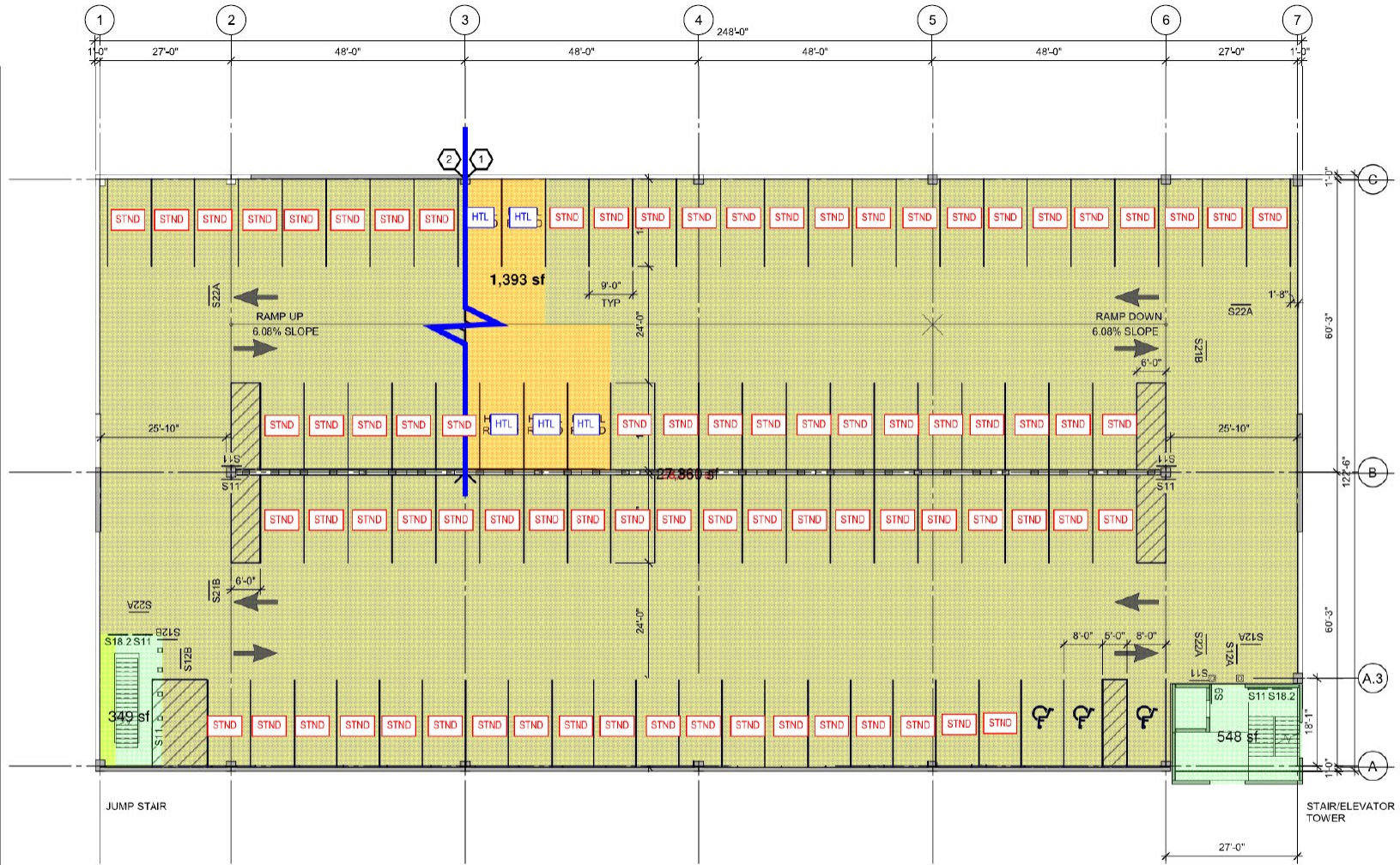
2 LEVEL 2 PLAN 1/16" = 1'-0"
