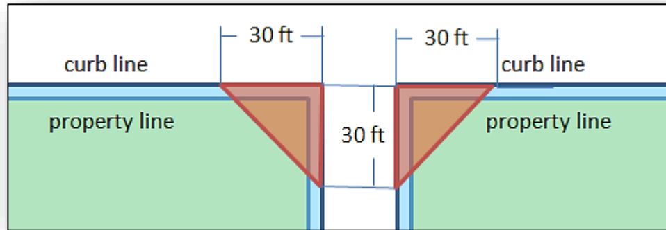
Figure 4.3: Sight Triangles
