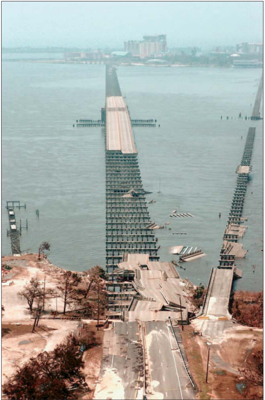
Wrecked bridges, Ocean Springs, MS Sun Herald news photo, Biloxi/Gulfport, MS
