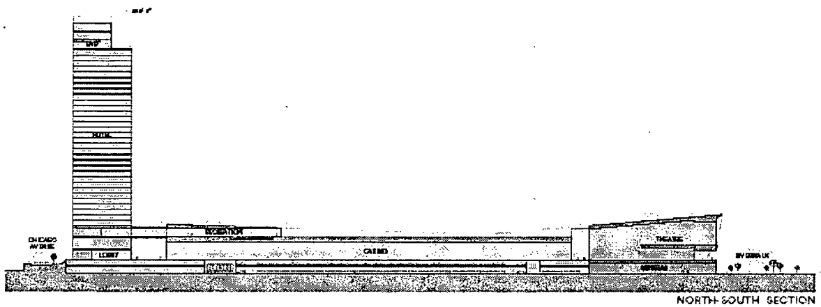
NORTH-SOUTH SECTION
