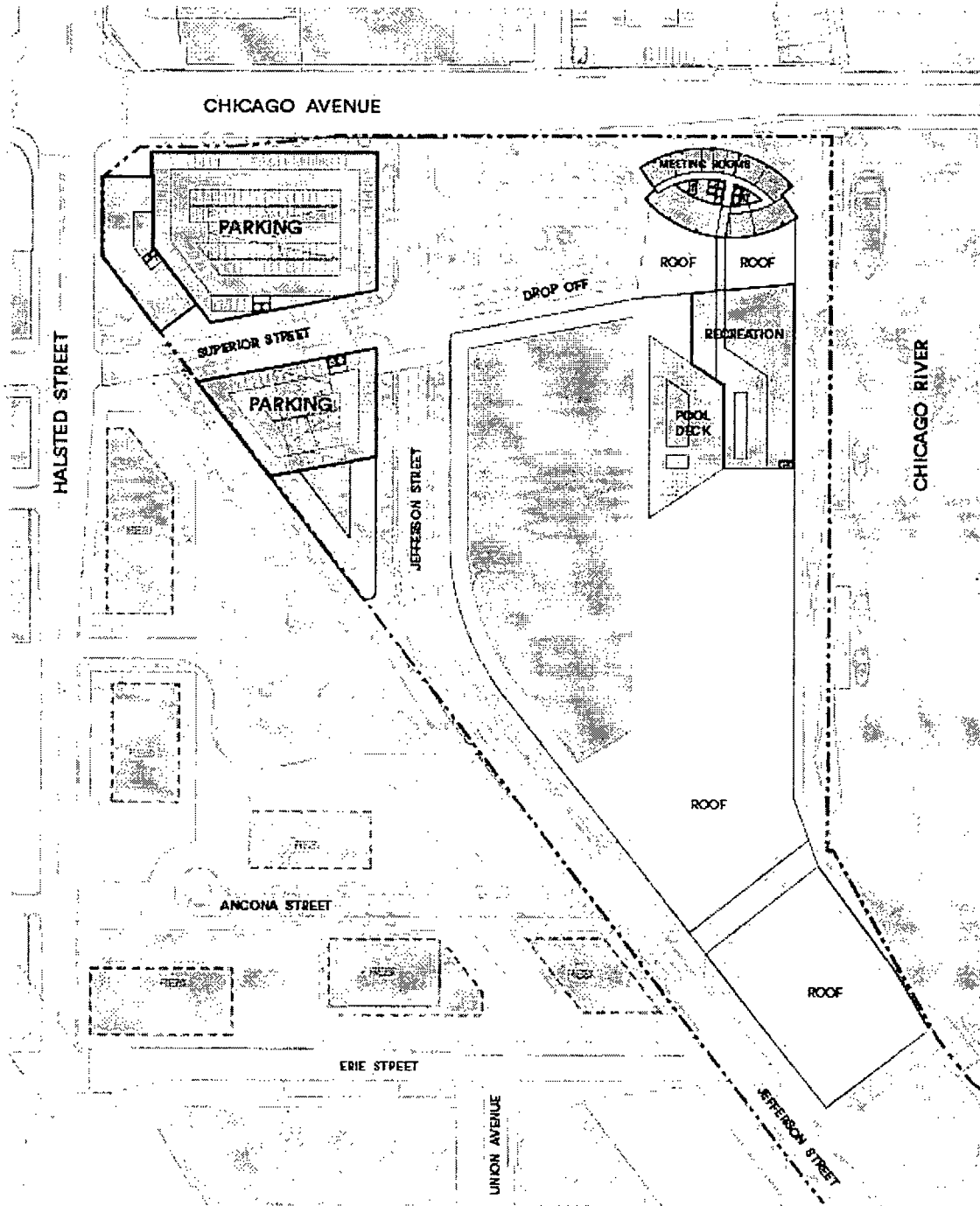
LEVEL 3 PLAN
