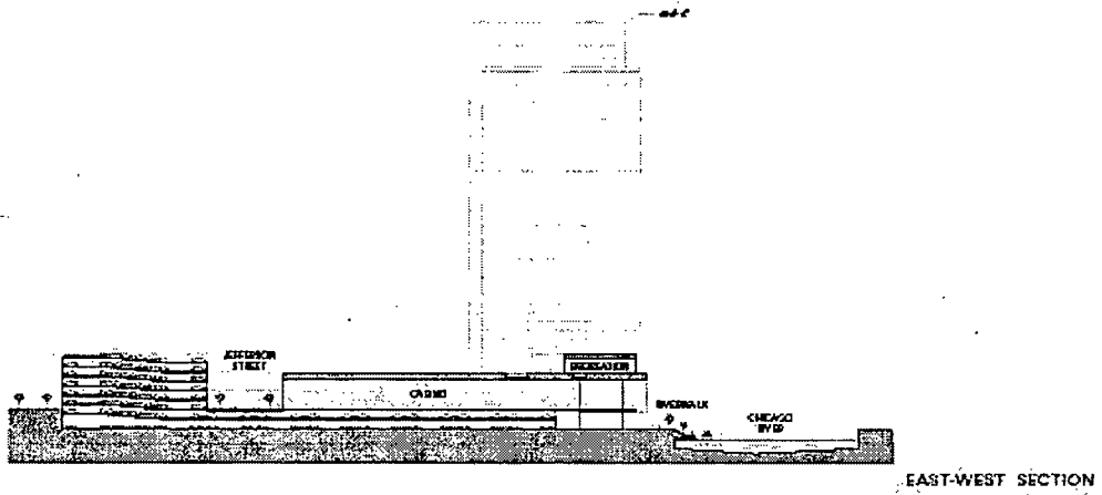
EAST-WEST SECTION
