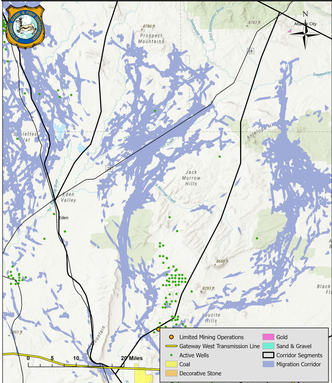
Figure 48. East of Farson Segment energy and mining development.
