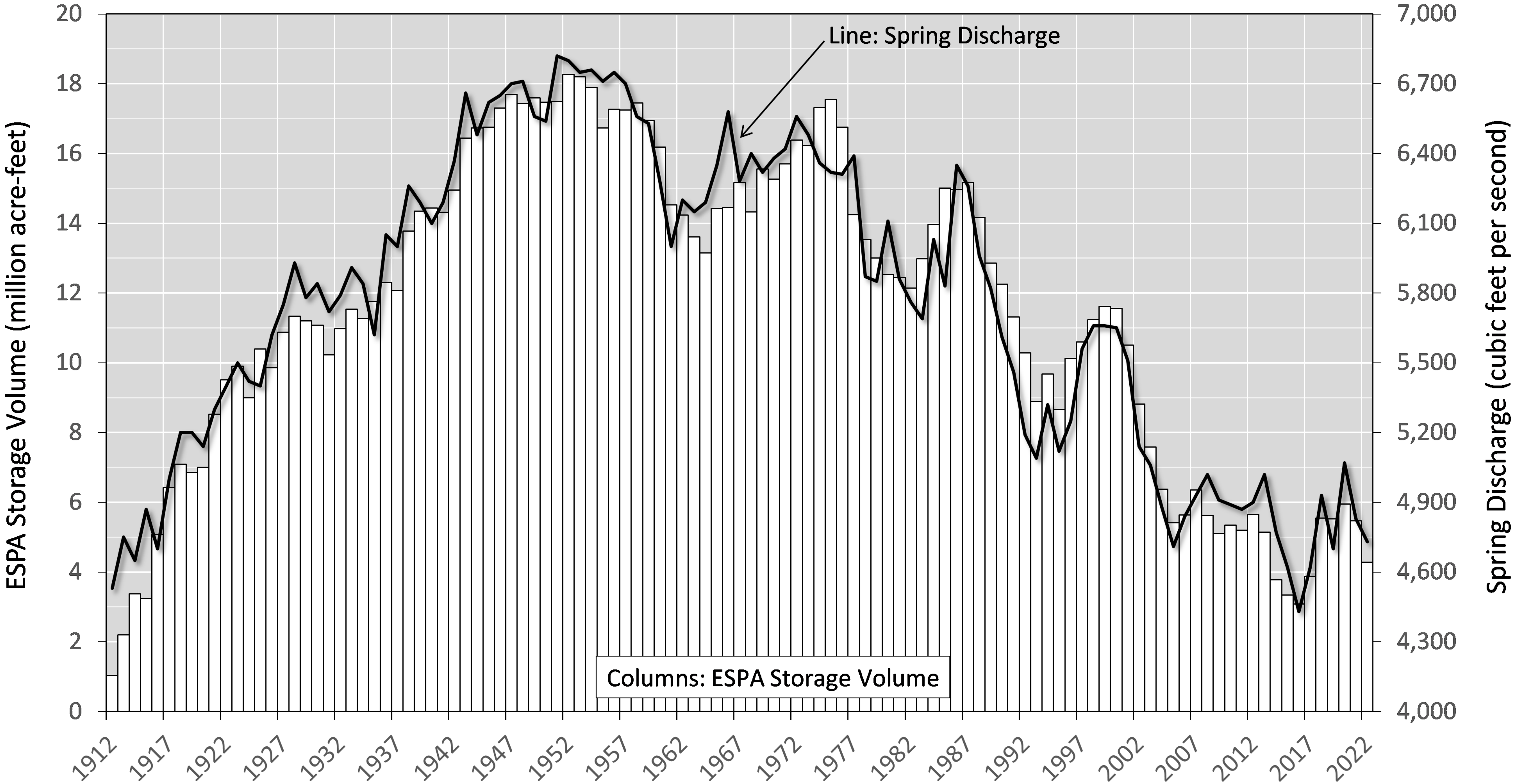
Annual ESPA Storage Volume Change and “Thousand Springs” Discharge
