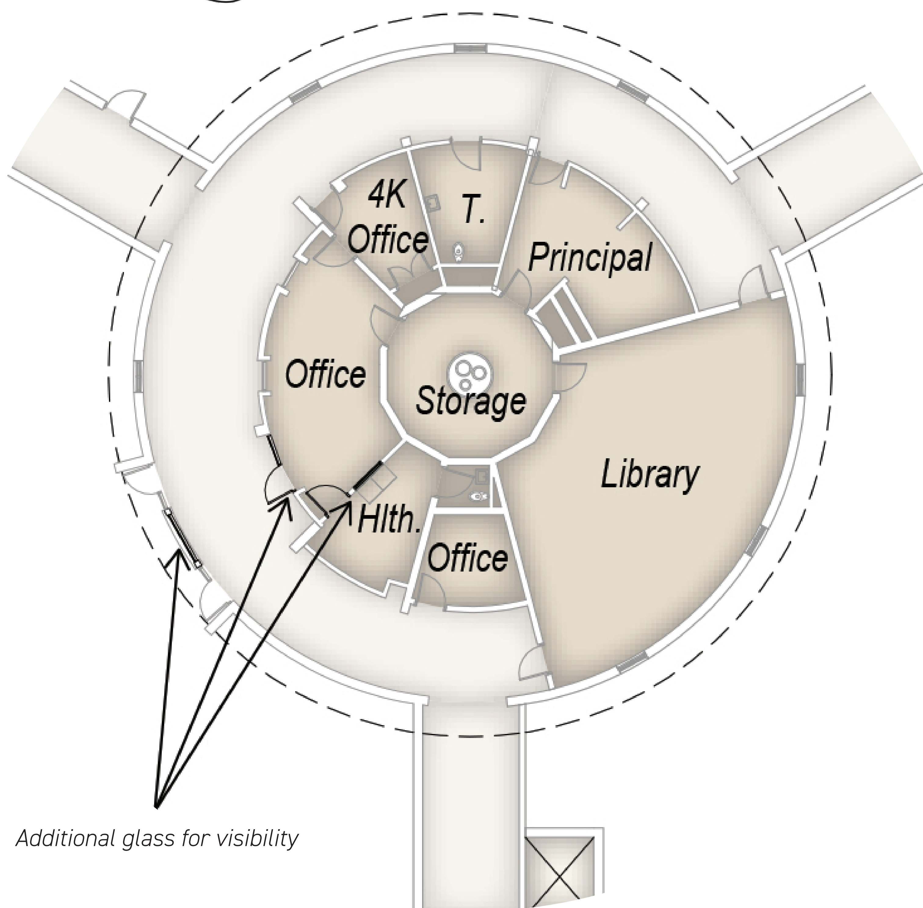
EARLY LEARNING CENTER SECURE ENTRY FLOOR PLAN
