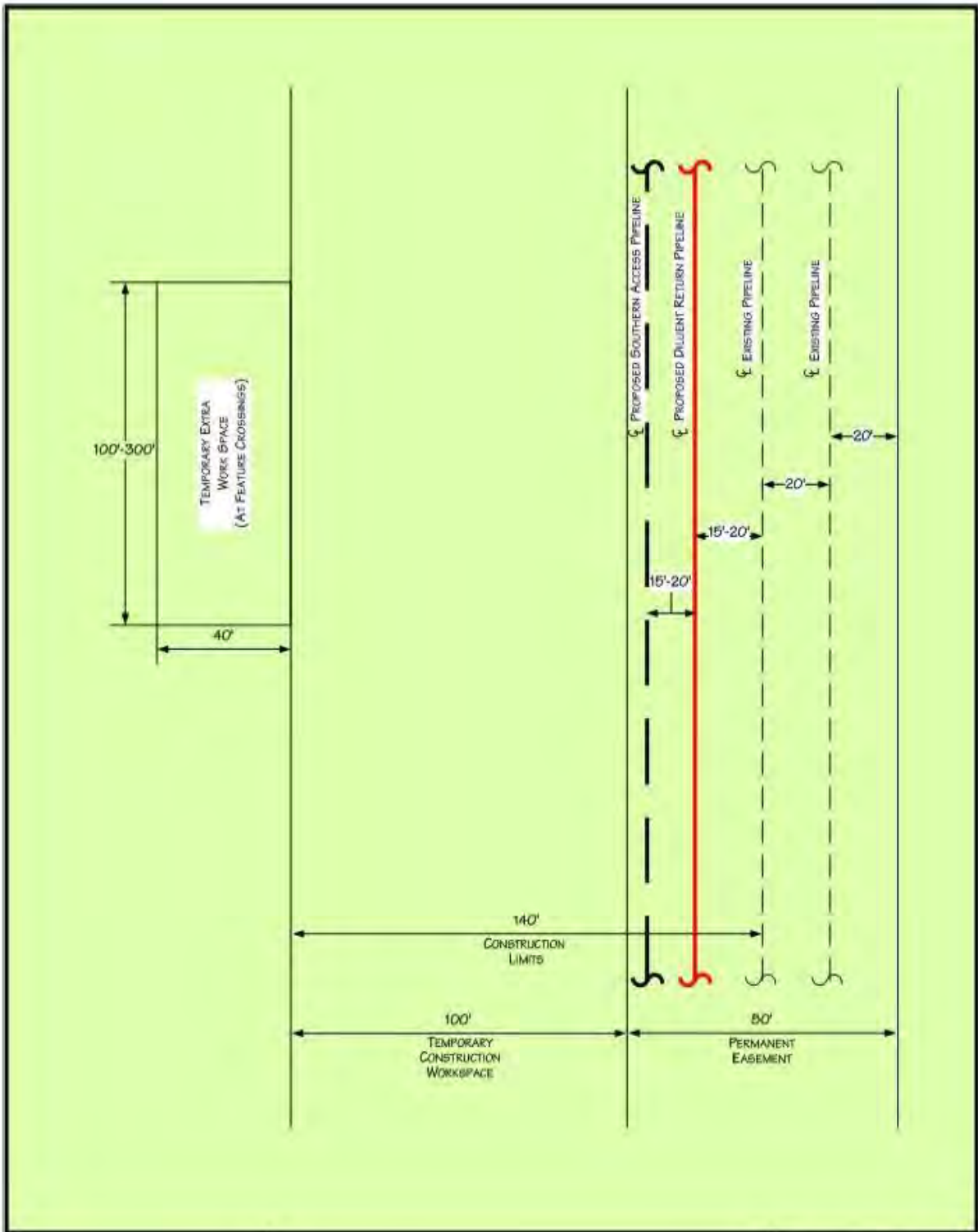
Figure 2 Typical Construction Layout and Workspace Configuration
