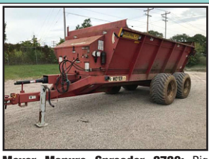
Meyer Manure Spreader 8720; Big 1000 PTO, Lights, Frt/Rear Splash guard, Self Oiler, Tongue Jack, Vertical Rear Beater, 550/45-22.5 tires. E40643. $17,299
