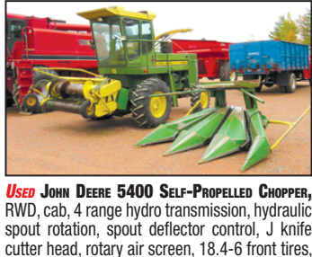
USED JOHN DEERE 5400 SELF-PROPELLED CHOPPER , RWD, cab, 4 range hydro transmission, hydraulic spout rotation, spout deflector control, J knife cutter head, rotary air screen, 18.4-6 front tires, 12.4-24 rear tires, 7 foot hay head with swivel gauge wheels, 3 row narrow corn head with row guides ..... $19,900
