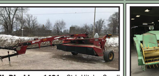
NH Discbine 1431; Std Hitch, Small 1000 pto, Lights, Rubber on Rubber Rolls, 13' Cut, Ten Pods, 31x13.50-15. E40041. .... $14,999
