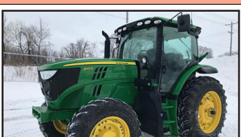
JD Tractor 6145R; CHA, 4wd, Instructor Seat, 6 Cyl Turbo, 145Hp, 7" Touch Screen, Auto Quad Plus 20F/20R Economy, 540/1000 pto, 3 Mech. Rmts, 3pt Top Link, DEF, 480/80R38. One Owner! E39893 ... CALL
