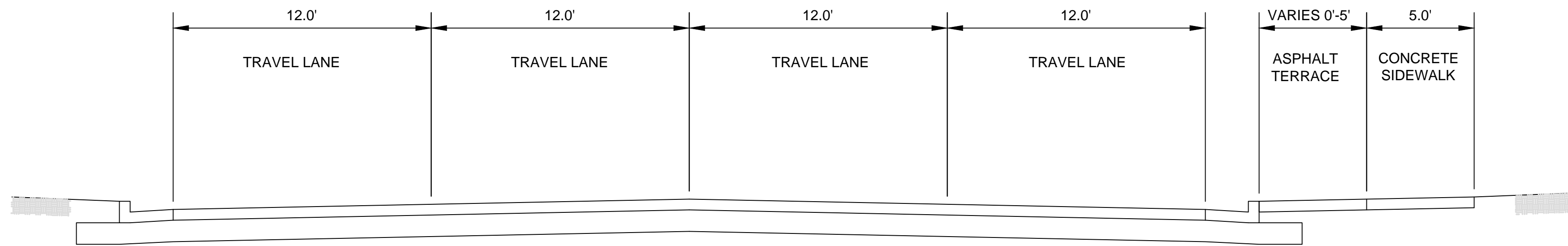
EXISTING TYPICAL SECTION BAINBRIDGE STREET TO ROSE STREET/COPELAND AVENUE
