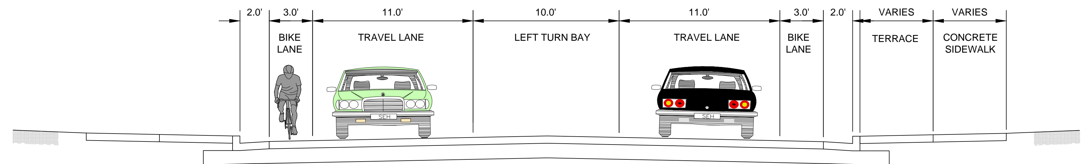
PROPOSED TYPICAL SECTION ROSE STREET/COPELAND AVENUE TO CALEDONIA STREET
