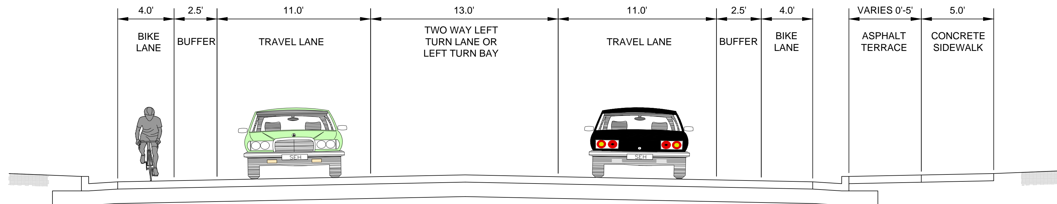
PROPOSED TYPICAL SECTION BAINBRIDGE STREET TO ROSE STREET/COPELAND AVENUE
