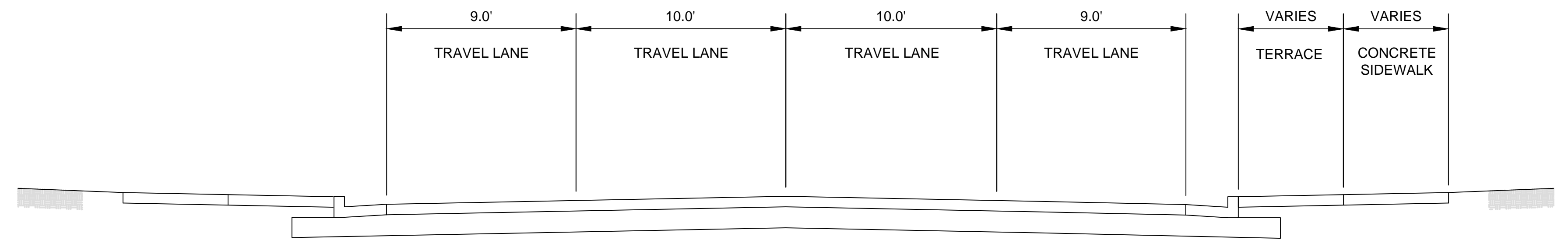
EXISTING TYPICAL SECTION ROSE STREET/COPELAND AVENUE TO CALEDONIA STREET
