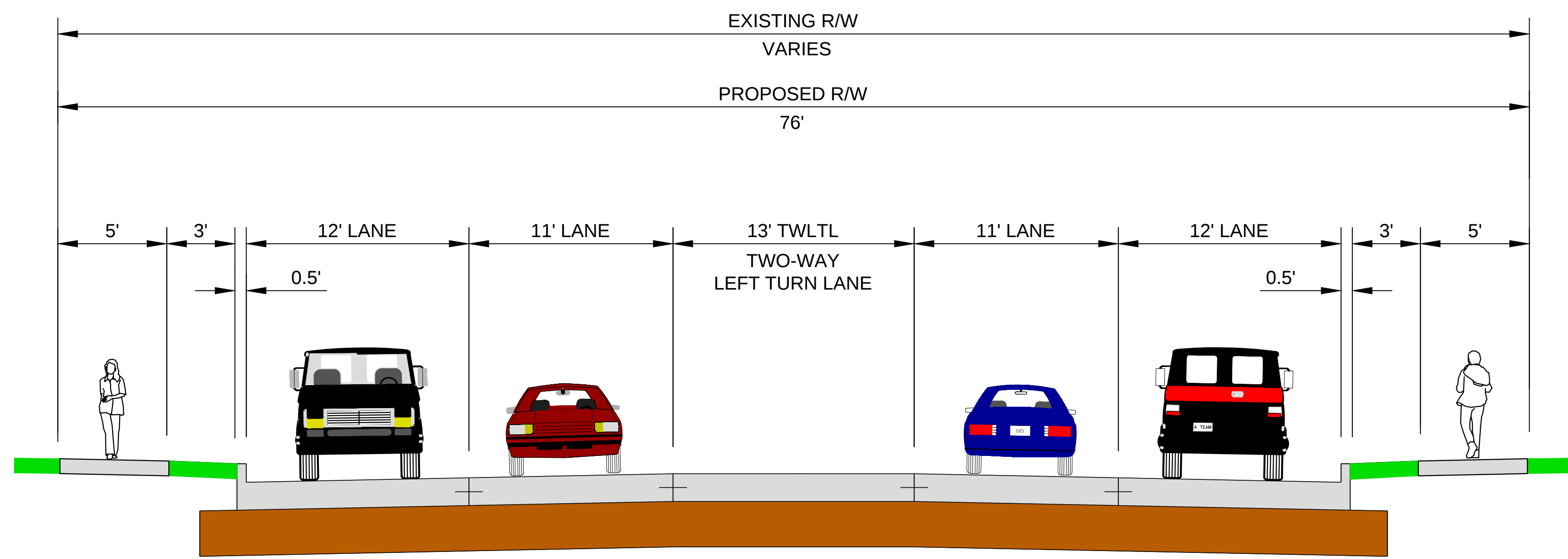
US 14 | SOUTH AVENUE - FINISHED ROADWAY
