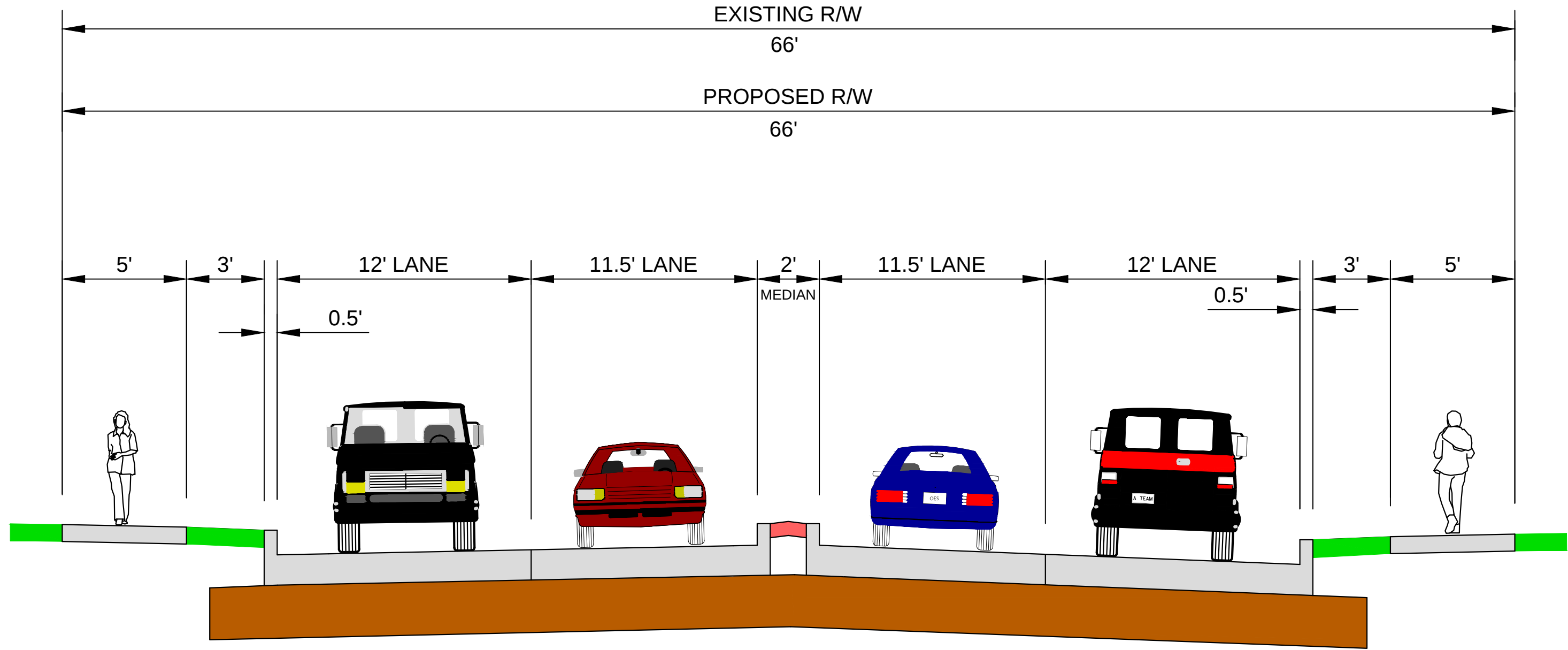
US 14 | SOUTH AVENUE - FINISHED ROADWAY
