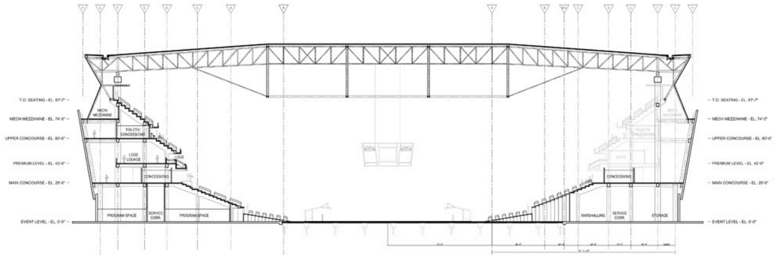
LONGITUDINAL SECTION - LOOKING WEST
