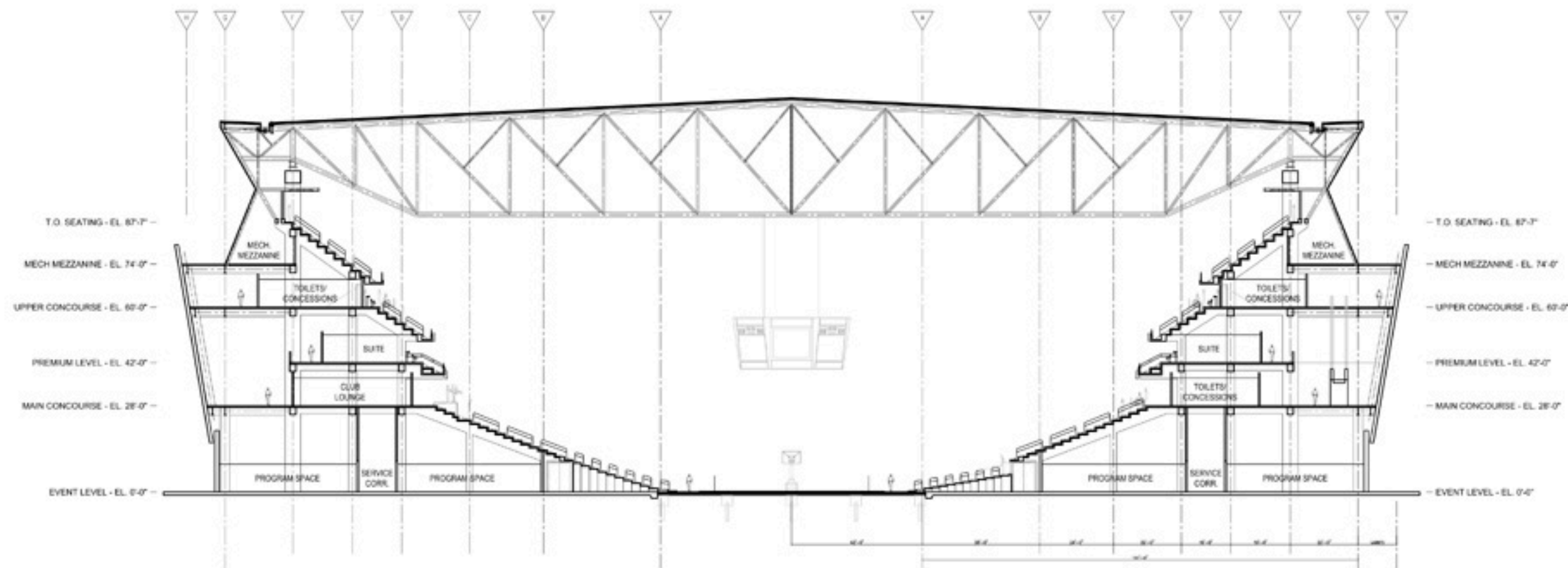
TRANSVERSE SECTION - LOOKING NORTH
