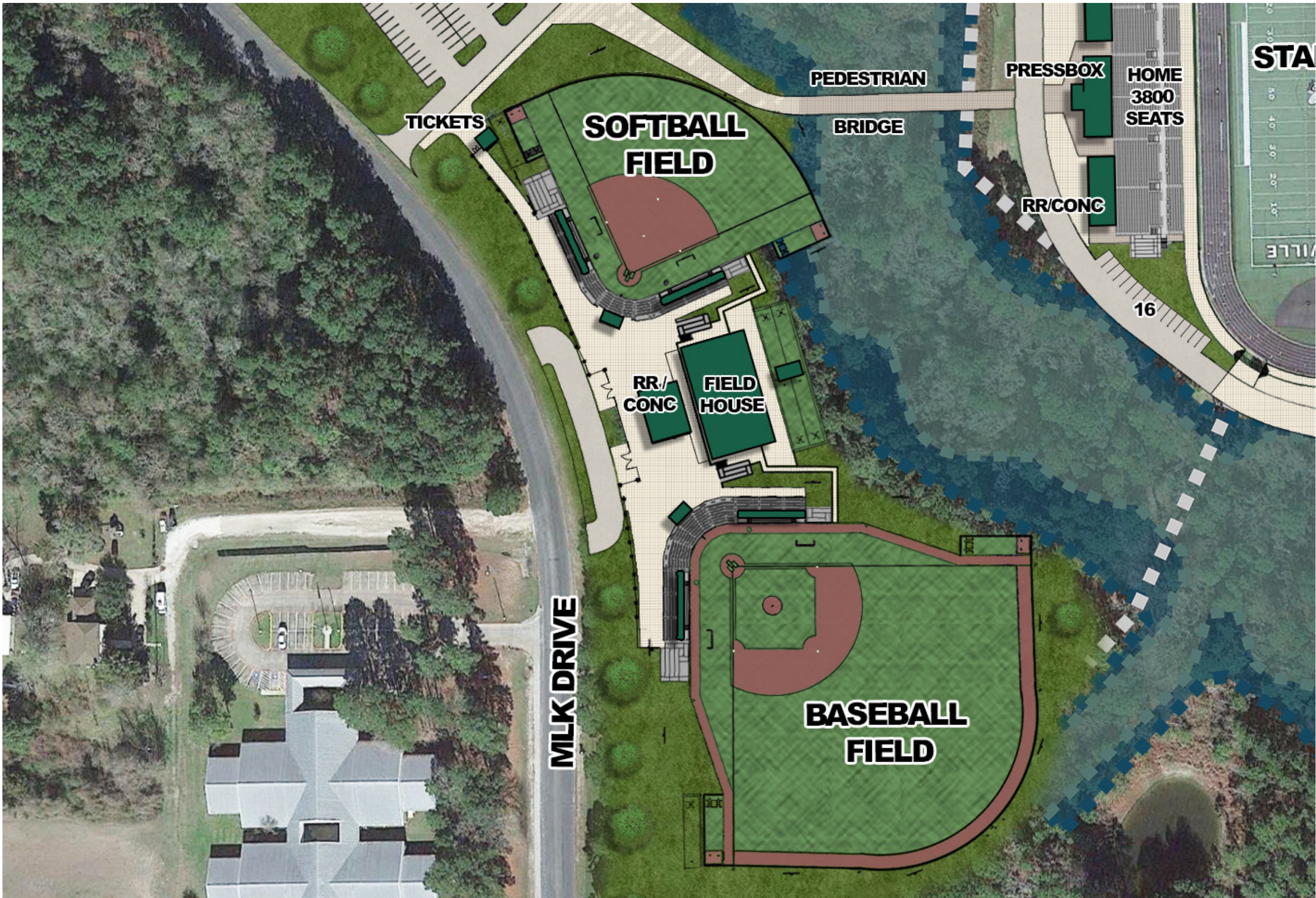
BASEBALL & SOFTBALL_ENLARGED SITE PLAN HUNTSVILLE ISD
