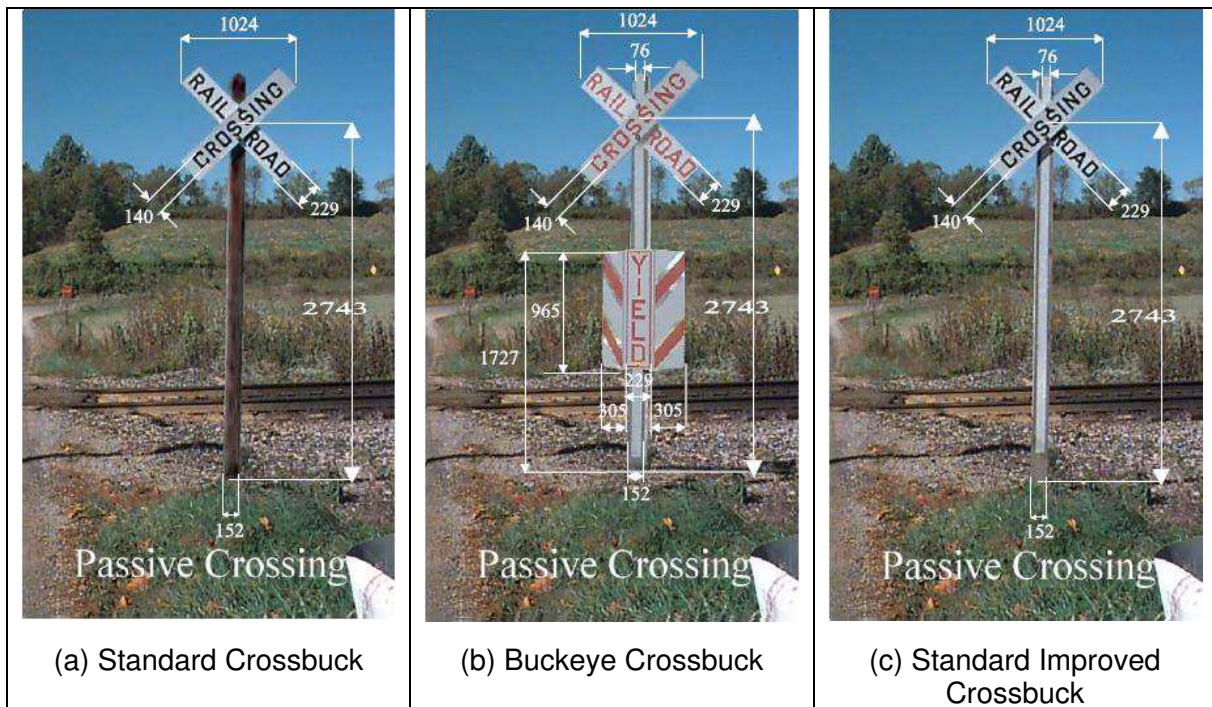
Figure 4. Crossbuck systems used in Zwahlen and Schnell (2000).
