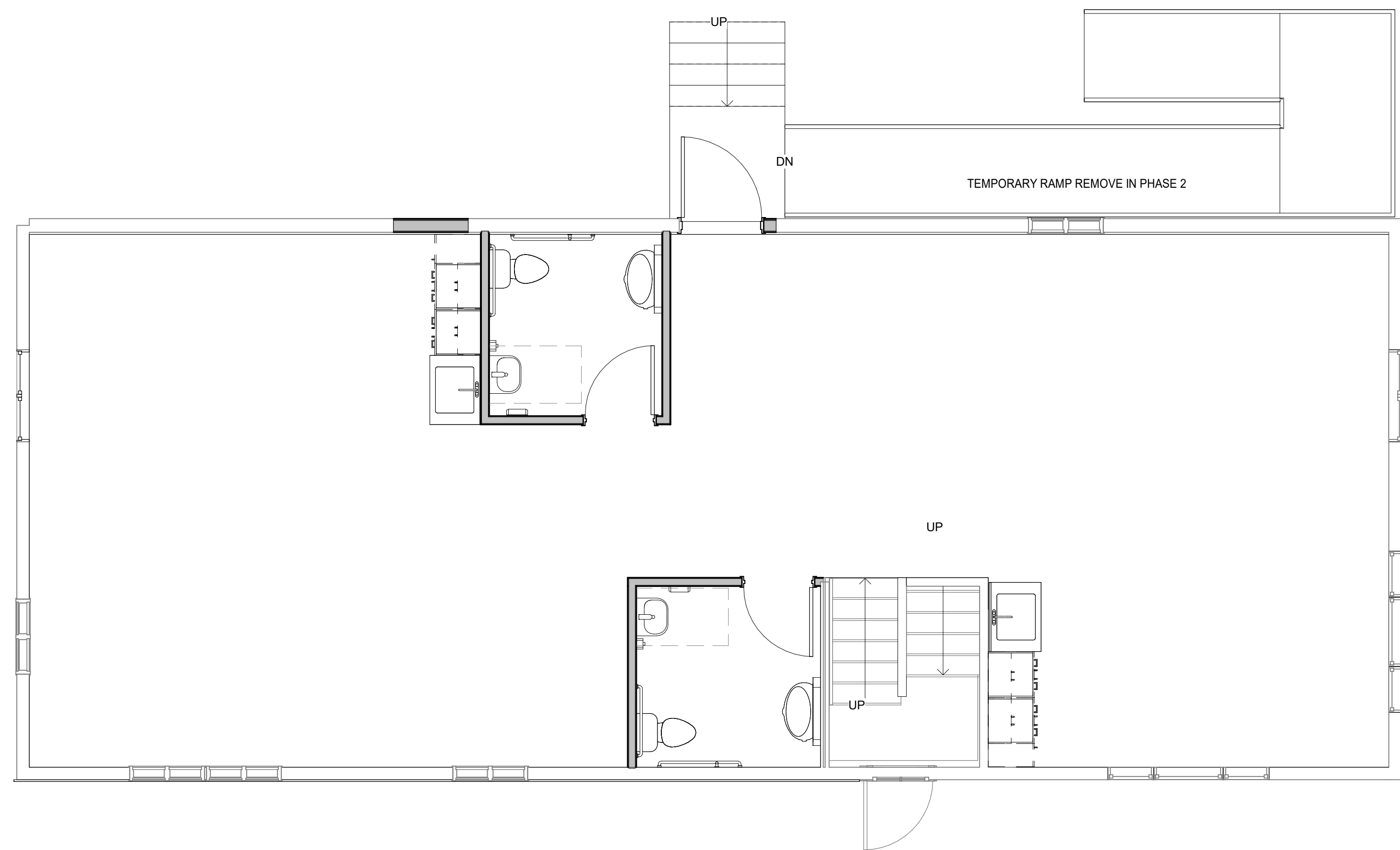
② PHASE 1 1/4" = 1'-0"
