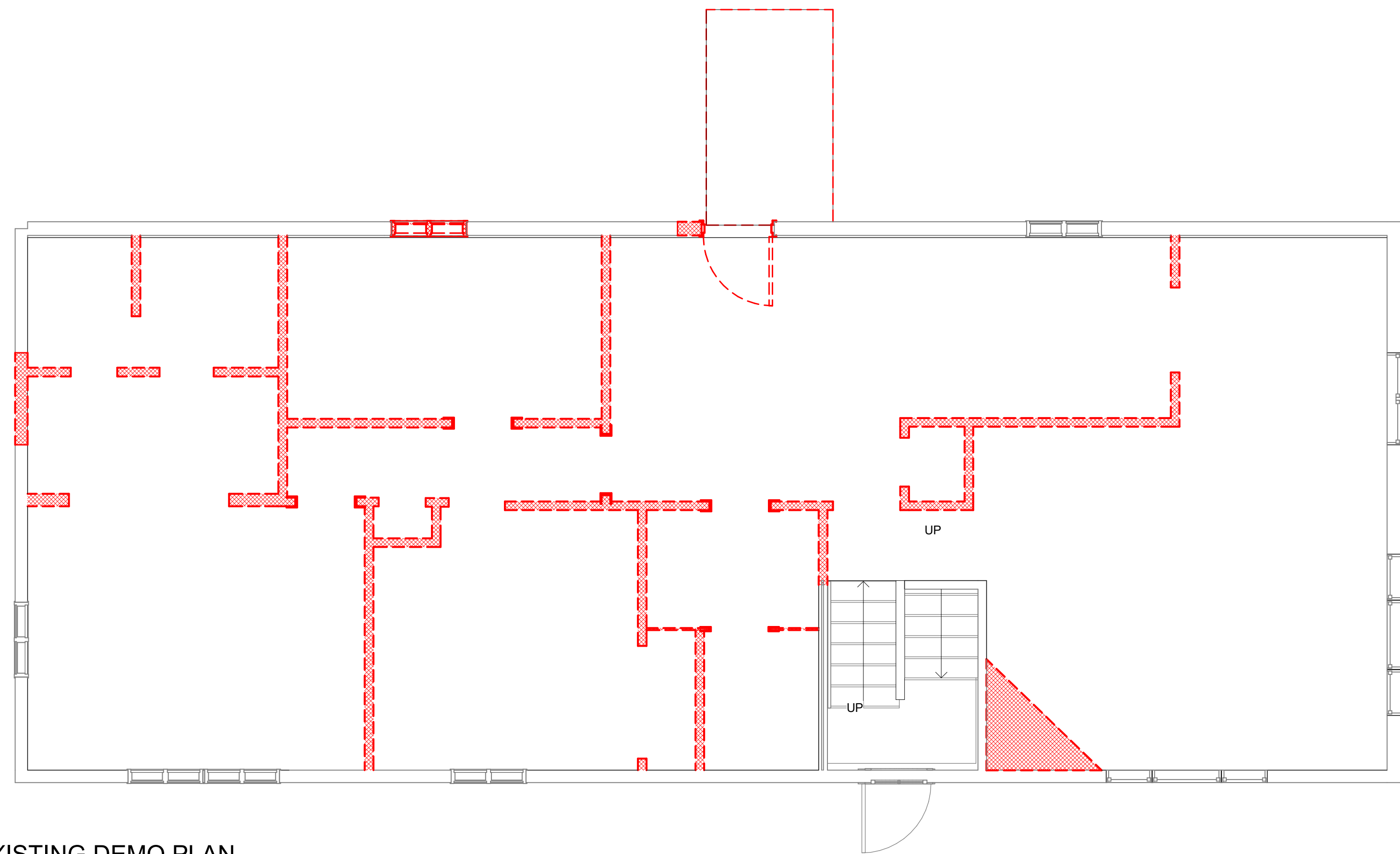
① EXISTING DEMO PLAN 1/4" = 1'-0"
