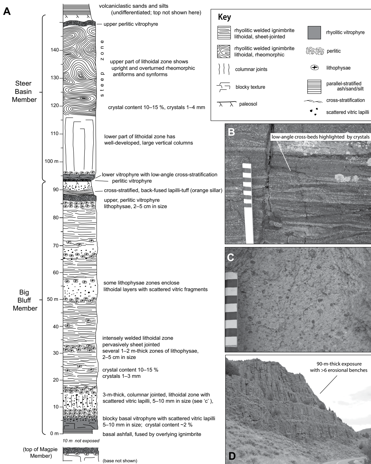
Figure 5. (A) Big Bluff and Steer Basin Members, at Magpie Basin ( 42^{\circ}15'01.3''\text{N} , 114^{\circ}15'51.2''\text{W} ). (B) Low-angle cross-stratification highlighted by crystals in the lower vitrophyre of the Steer Basin Member. (C) Abundant scattered angular vitric fragments supported in tuff matrix in the lower lithoidal zone of the Big Bluff Member. (D) Big Bluff Member in Rock Creek Canyon: Benches mark successive lithophysal zones showing the compound nature of the ignimbrite.
