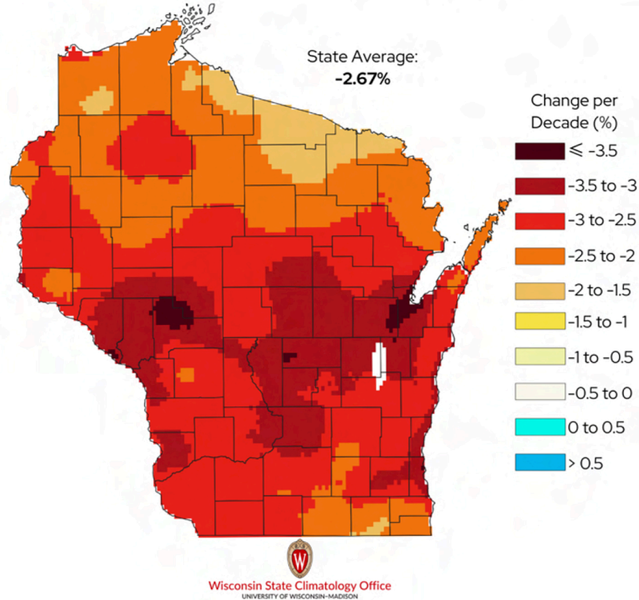
Figure 4. The percent change per decade in the number of March hours at or below freezing across Wisconsin from 1951 to 2024. Most of the state has experienced a two to three percent decline per
