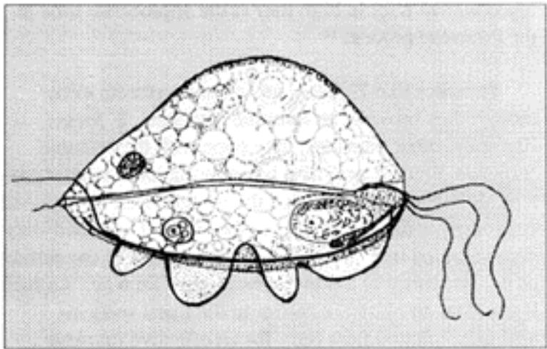
Figure 1. Trichomonads exhibit three anterior flagella, a single posterior flagellum, and an undulating membrane.
