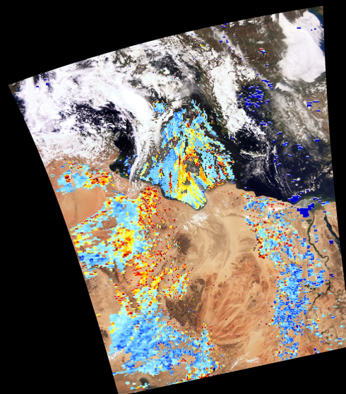
Aerosol Layer Height 0.0 2.0 4.0 6.0 8.0
