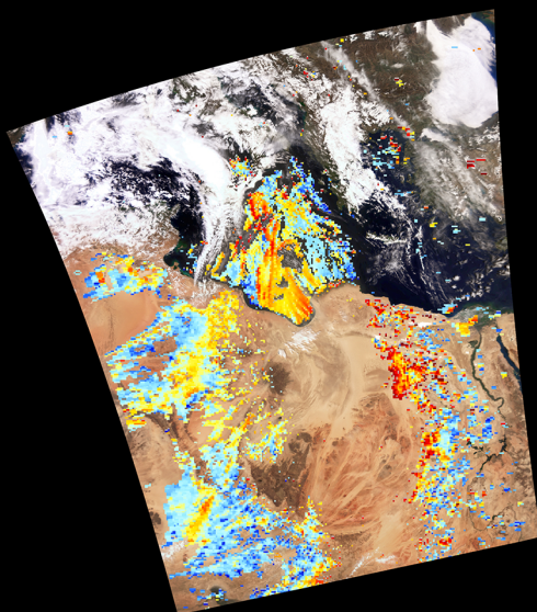
Single Scattering Albedo (SSA) 0.55 \mu\text{m} 0.80 0.84 0.88 0.92 0.96 1.00
