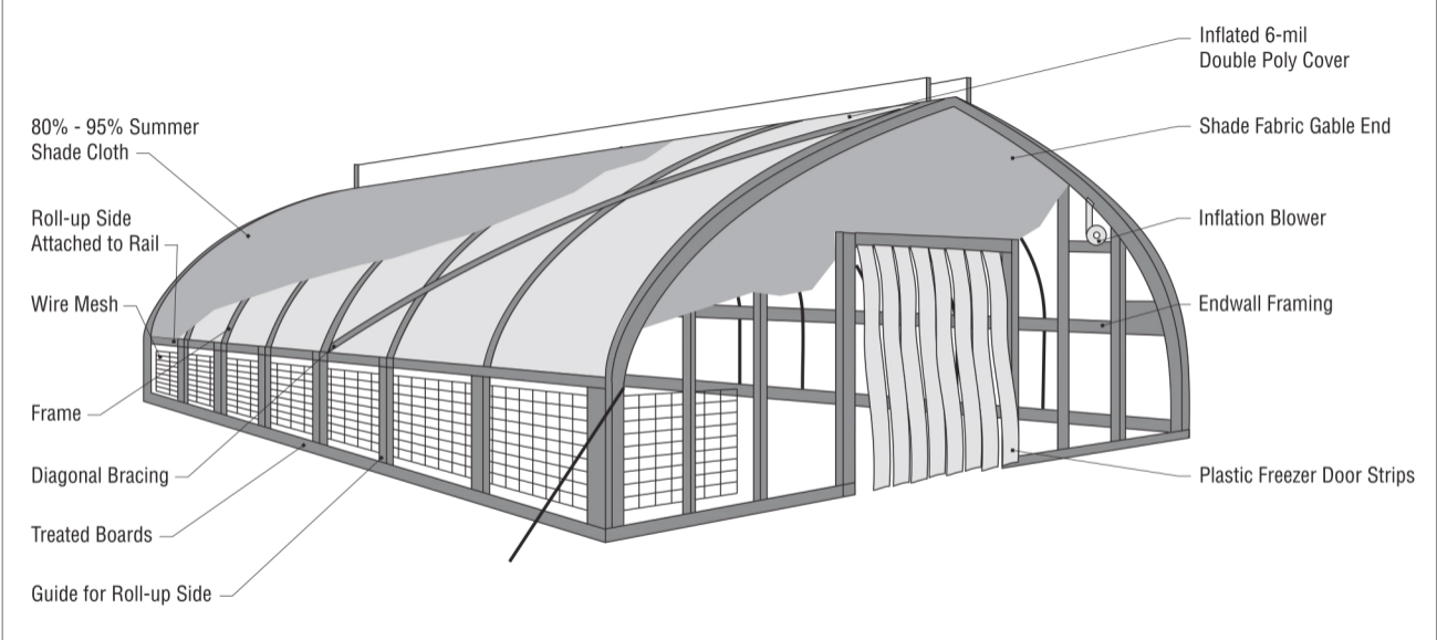
Figure 1. Basic components of a greenhouse barn
