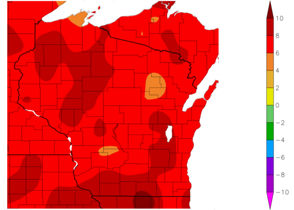
Departure from Normal Temperature (F) 9/21/2025 – 10/20/2025
