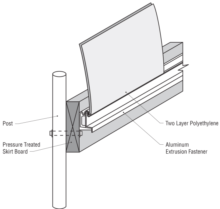
Figure 5. Common method of anchoring plastic covers.
