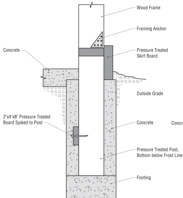
4b. Post frame.
