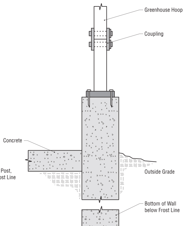
4c. Concrete pier.
