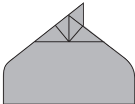
2d. Gable Frame with Overshot Ridge.
