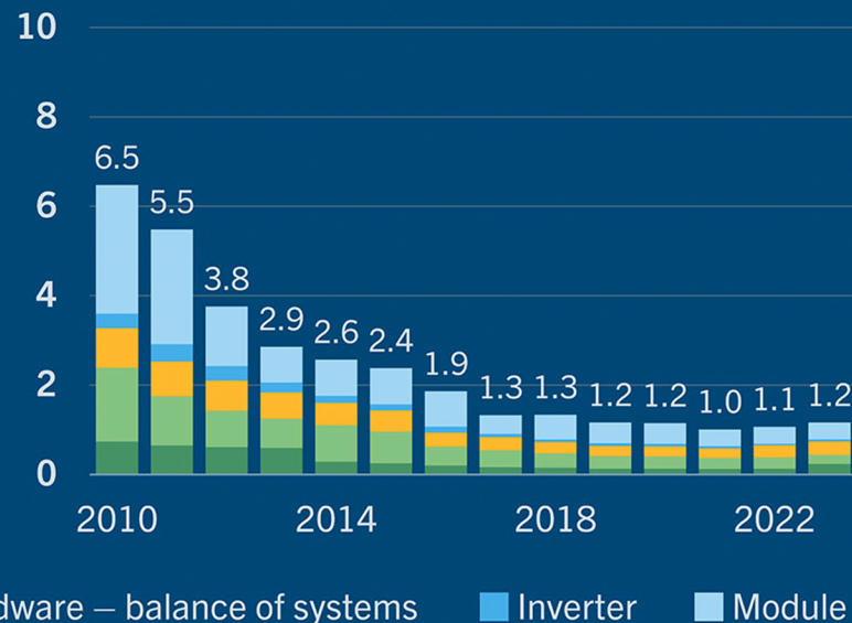
Utility-scale solar cost (dollars per Wdc)
