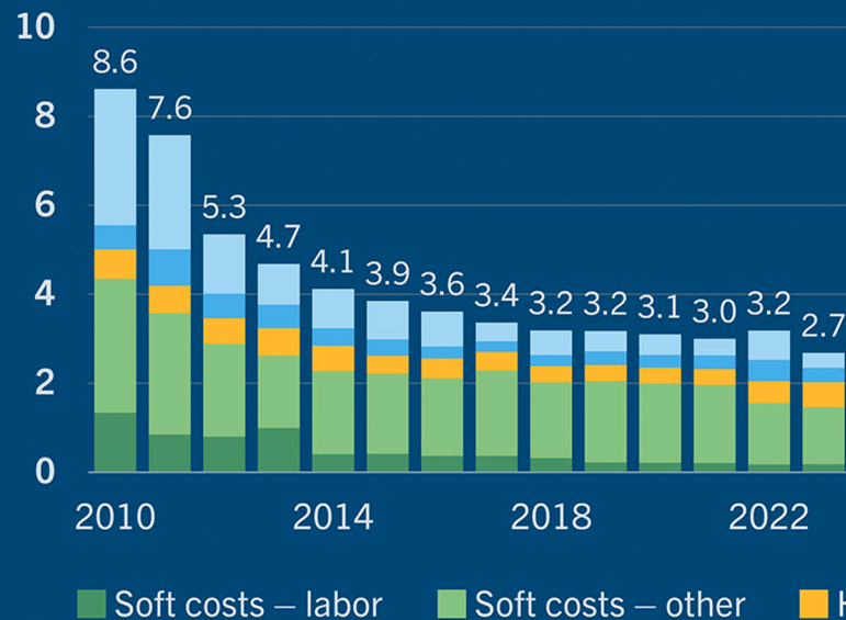
Residential solar cost (dollars per Wdc)
