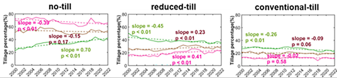
Figure 5(b). Temporal trends of tillage percentage for region A, B, and C (see color scheme in (a))
