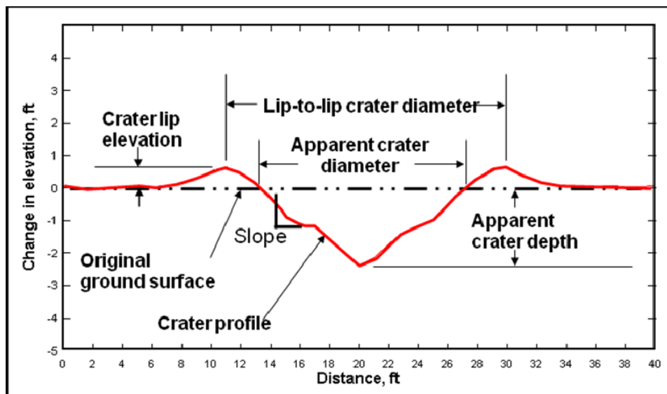
Figure 49. WFC Explosion Crater Profile Measurements (Source: Army Corps of Engineers)
