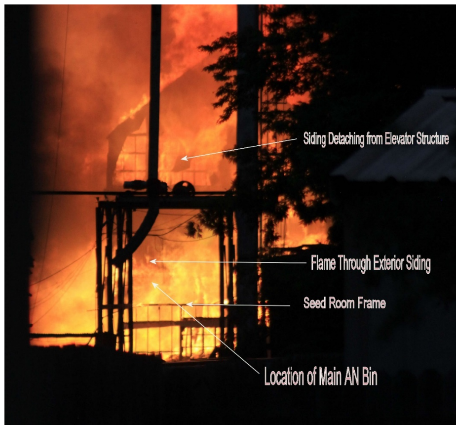
Figure 43. North Side of Structure Approximately 3 Minutes Before Detonation, with Dark Foreground Objects Associated with the Bin Complex North of Fertilizer Building (Source: Member of the Public)
